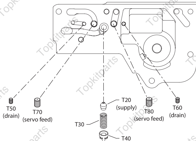
View "A"
