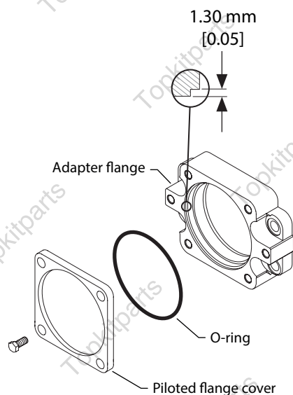
Old design
