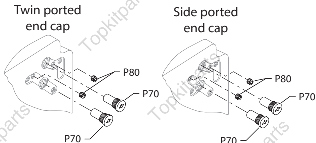
View "A" with pressure limiters, left hand rotation, (1, 5 & 6)
