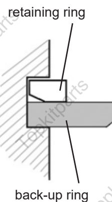
22. Assemble the retaining ring. Make sure the chamfer is downwards.
