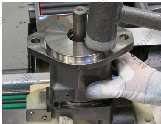
17. Carefully tap down the bearing housing.
