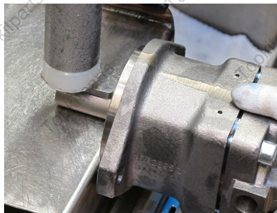
24. Tap down the flat key and turn the shaft at least one revolution. Make sure the back-lash of the gears are correct (see page 12).
