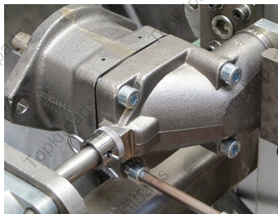
23. Assemble the hexagon screws and torque them to specified value, shown on page 12.
